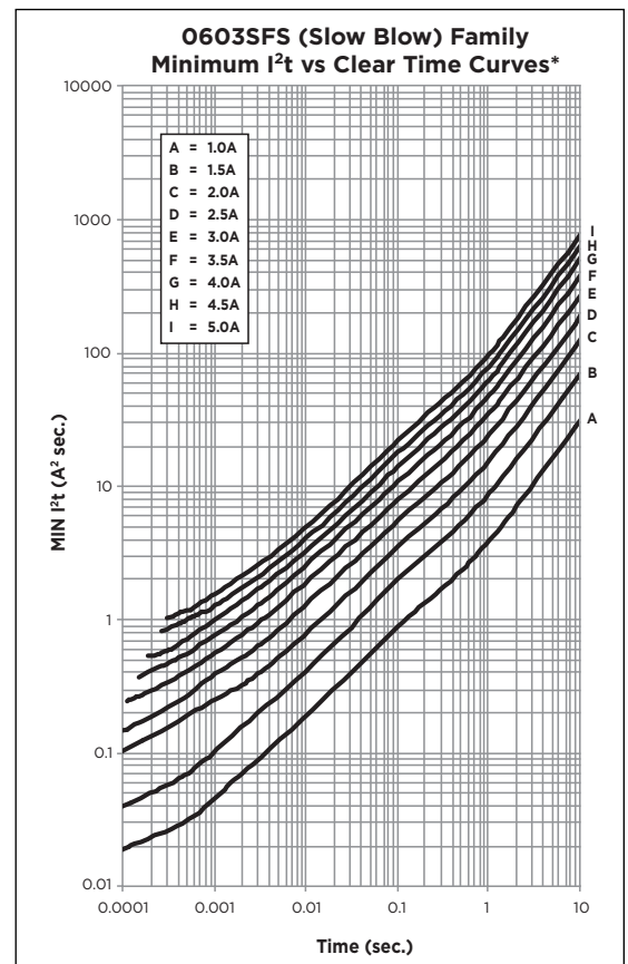
Figure 6. O603SFS (Slow Blow) Family Minimum I^2t vs Clear Time Curves
